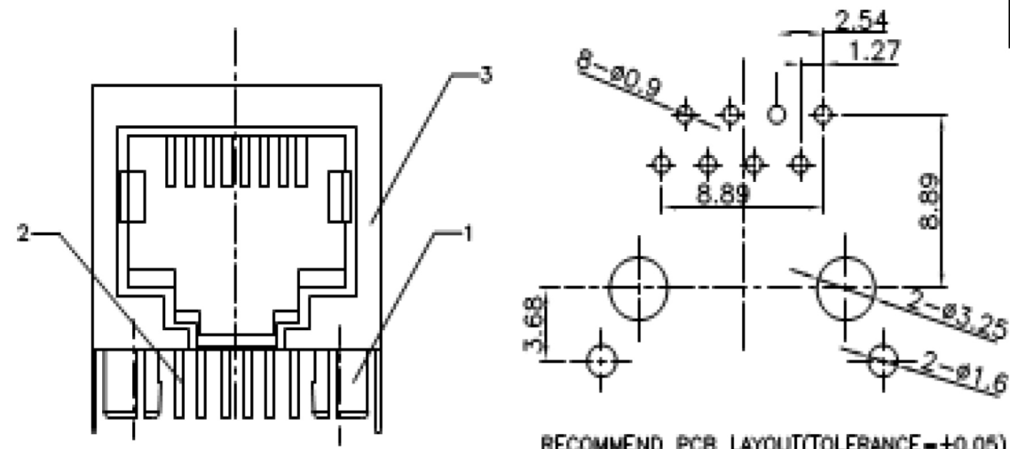
RECOMMEND PCB LAYOUT(TOLERANCE=±0.05)
